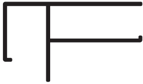
Gable End Rafter - DynaGlas
