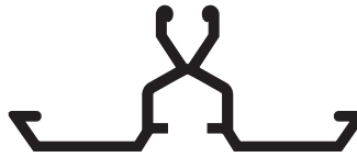
Support Rafter - 8mm
