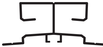
Ridge - Arched - 8mm
