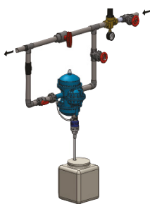
bypass installation
